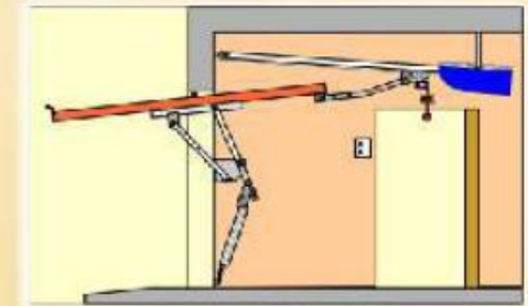
Spring Balanced Tip-up Doors
