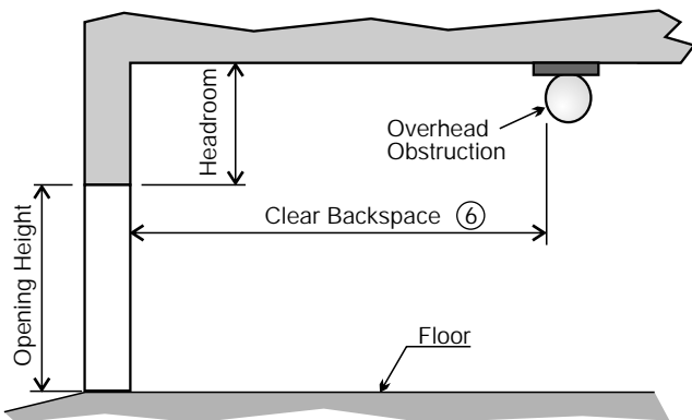
Cross-Section Through Garage
